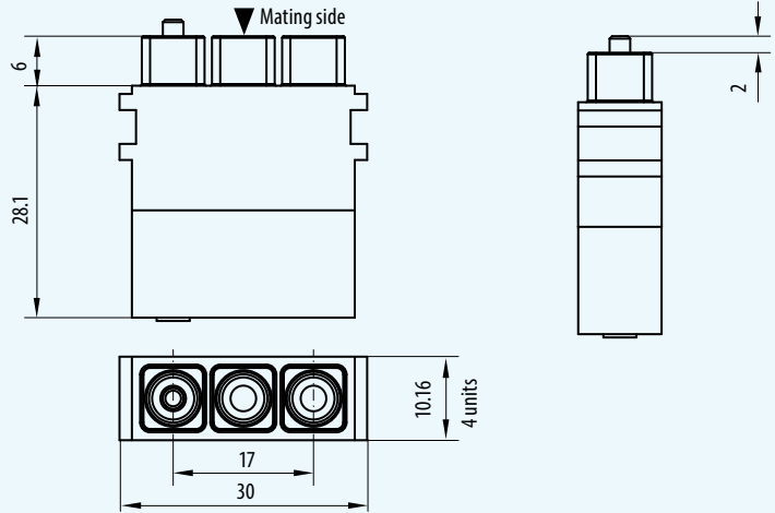
Insulator pin
