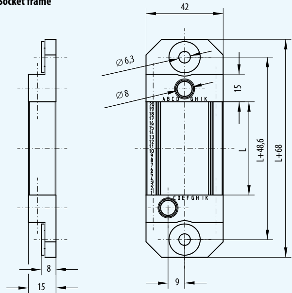
Socket frame
