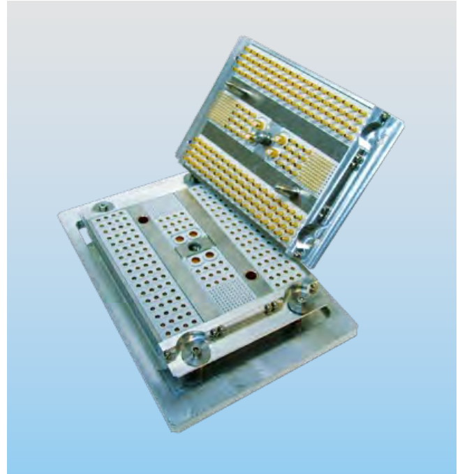
Complete docking unit. Three ODU-MAC series units, including special spindle locking, are assembled into a special frame made of stainless steel.
