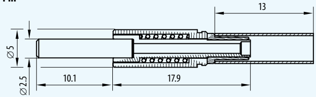
Pin
