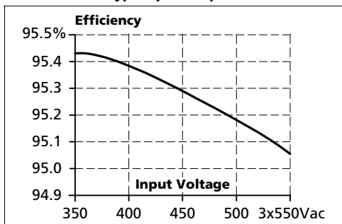
Fig. 10-3 Efficiency vs. input voltage at 48V, 20A, typ., 3-phase operation
